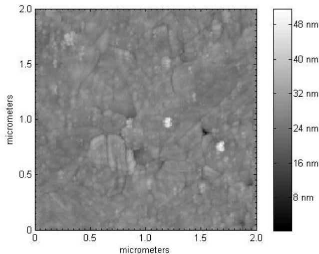
Figure 3 - Sample F (Courtesy of the Reifenberger Nanoscale Physics Lab at Purdue University)
