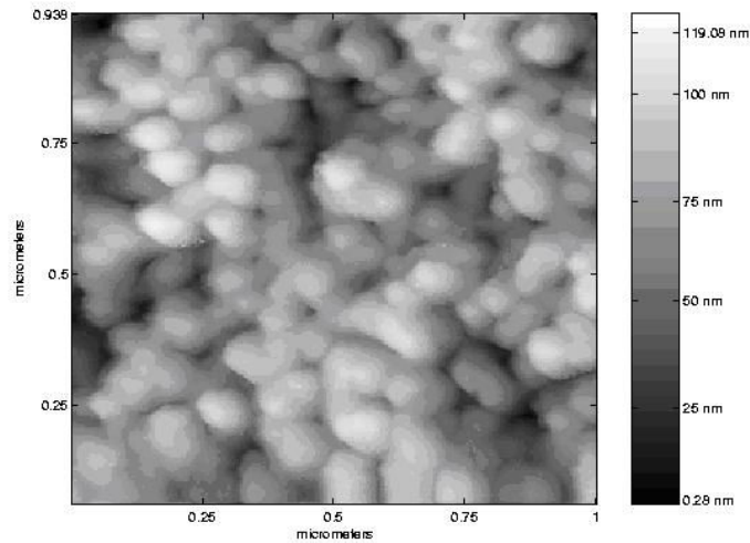
Figure 2 - Sample B (Courtesy of the Reifenberger Nanoscale Physics Lab at Purdue University)
